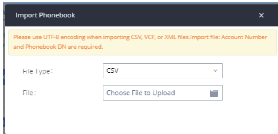
Figure 6: Import Phonebook
