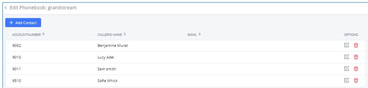
Figure 5: LDAP Entries
