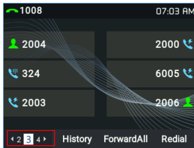
Figure 1: VPK Pages
