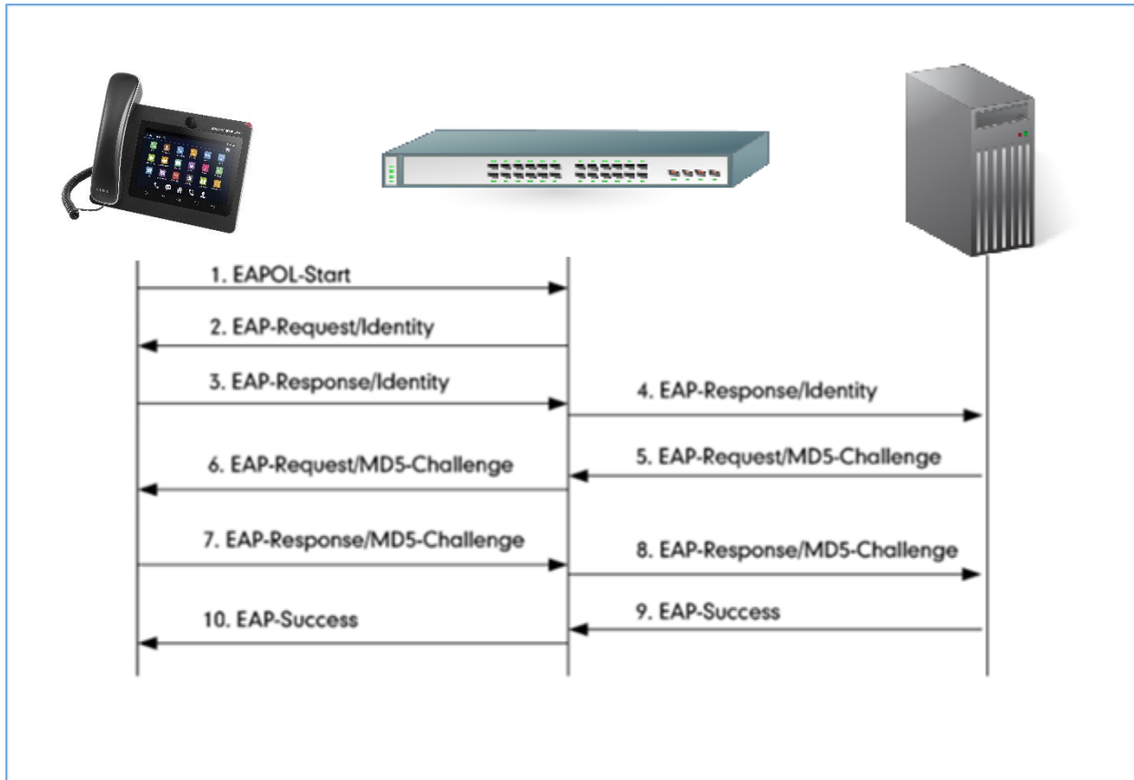
Figure 6: 802.1x Authentication Using MD5
