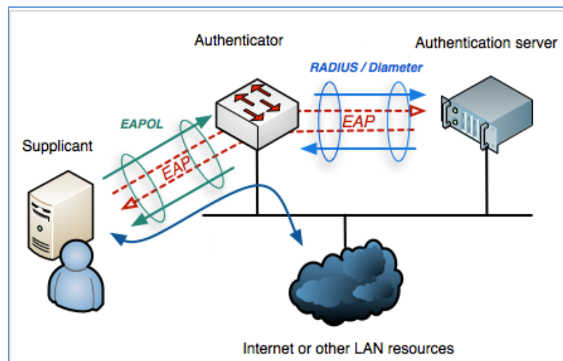
Figure 1: 802.1x Authentication Process
